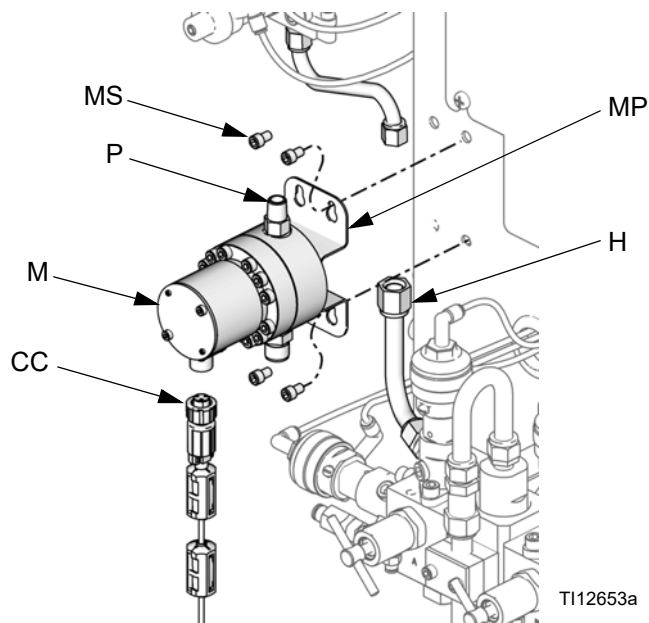
AFB. 23: G3000/G3000HR/G3000A debietmeters
