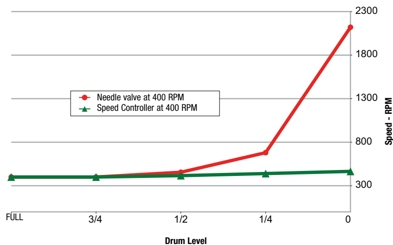
Speed Controller versus Needle Valve
