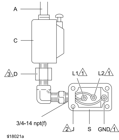
Figure 7 连接电源线
