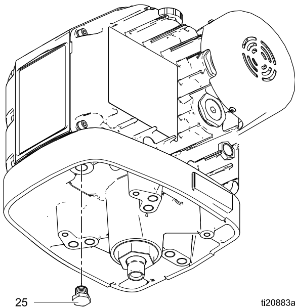
Figure 14 Oljedräneringsplugg
