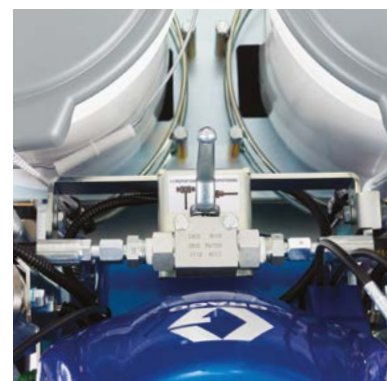
1:1 Hydraulic Proportioner
