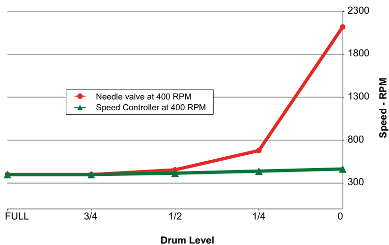
Speed Controller versus Needle Valve
