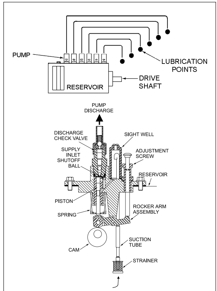
PUMP-TO-POINT SYSTEM
