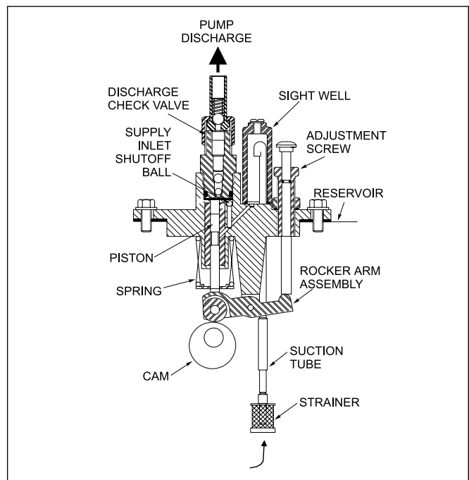
Pumps With Sight Glass
