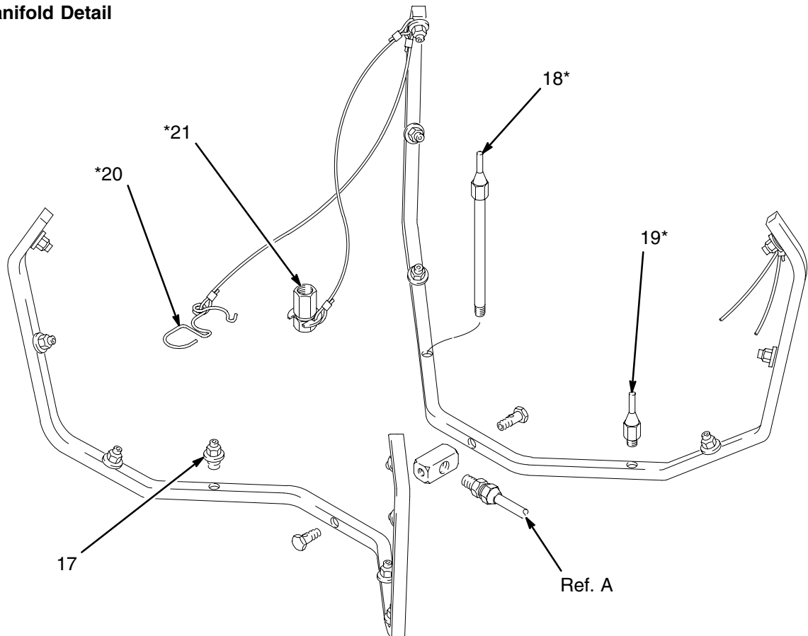
Fluid Manifold Detail
