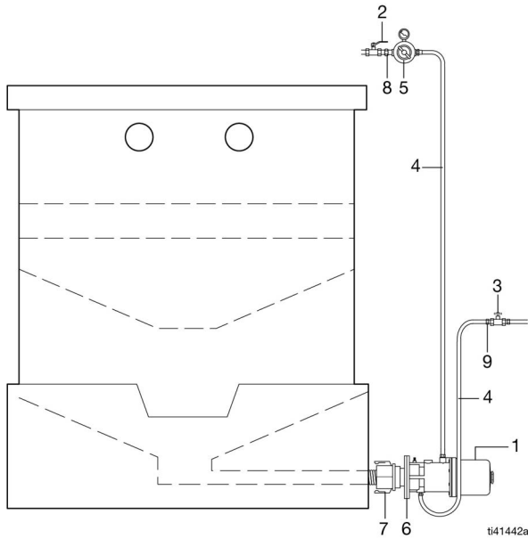
Horizontal Mount
