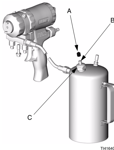
FIG. 4. Container Air Valve (Model 248139)
