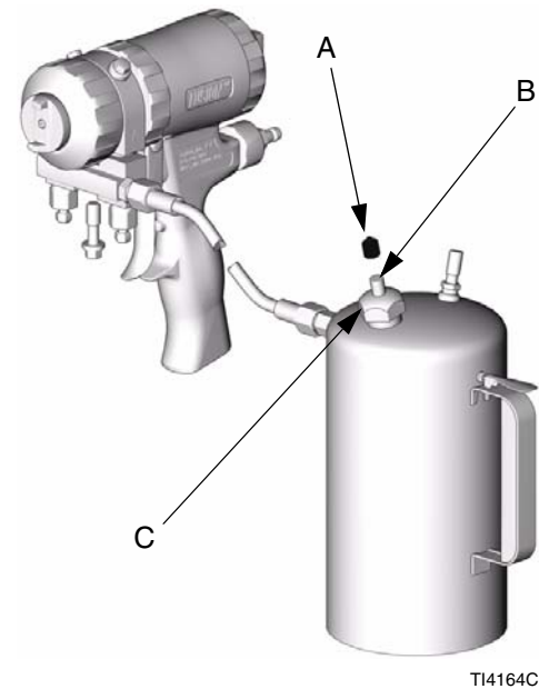
FIG. 4. Container Air Valve (Model 248139 Shown)
