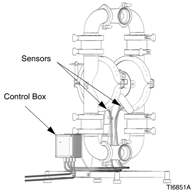
FIG. 3. Typical Installation
