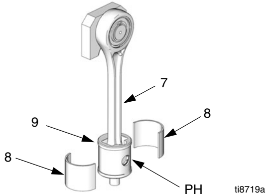
FIG. 4. Slider Bearings
