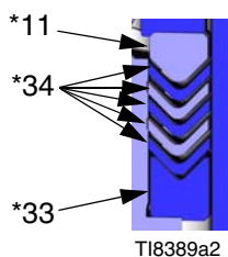
Piston Packings
