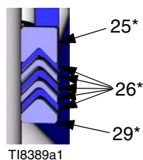
Throat Packings
