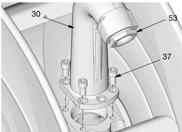
FIG. 62: Low Pressure Outlet shown. Medium Pressure models use 6 bolts.
