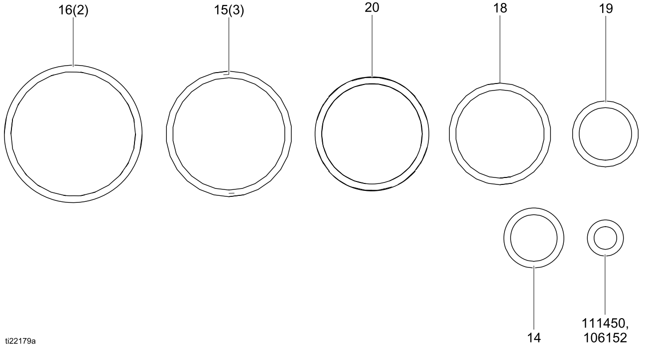
FIG. 6: Kit 24T848 and Kit 24Y671 O-Ring Sizes
