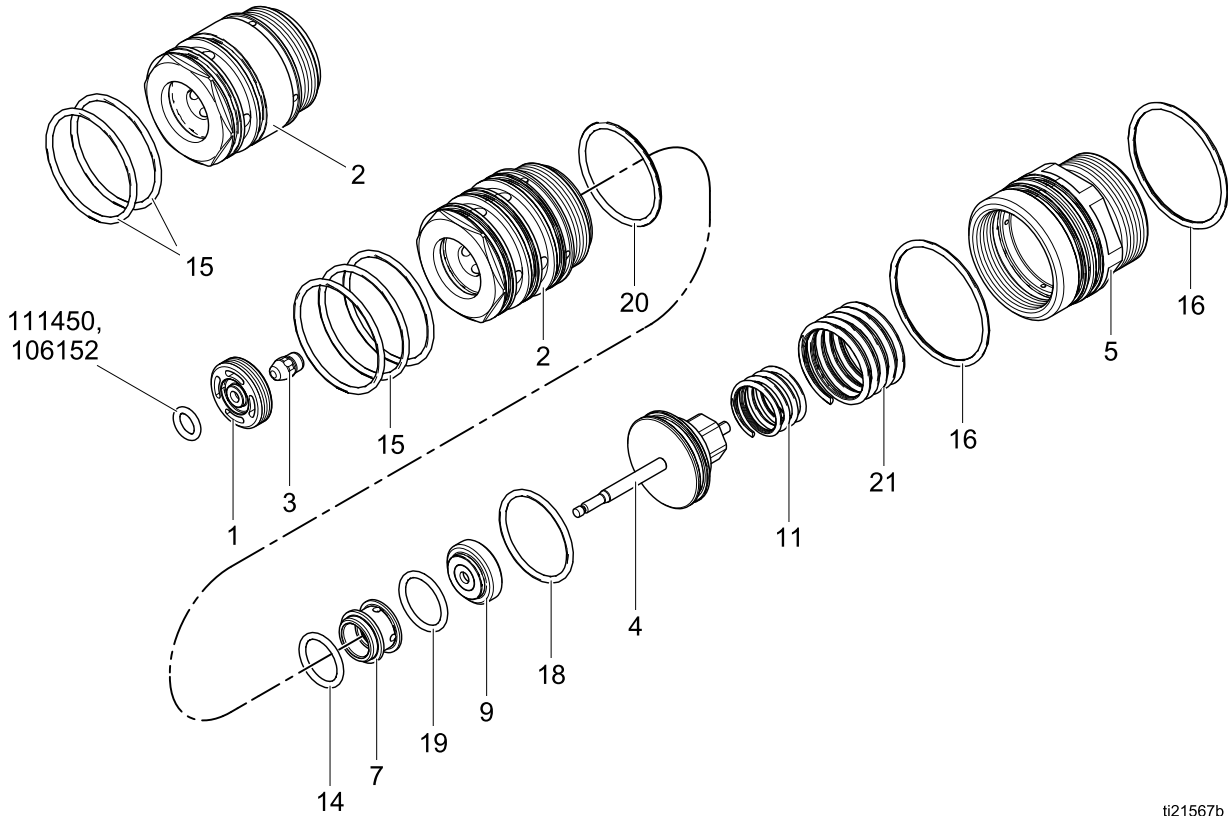
Fig. 2: Valve Assembly (High Pressure Circulating Valve Shown)
