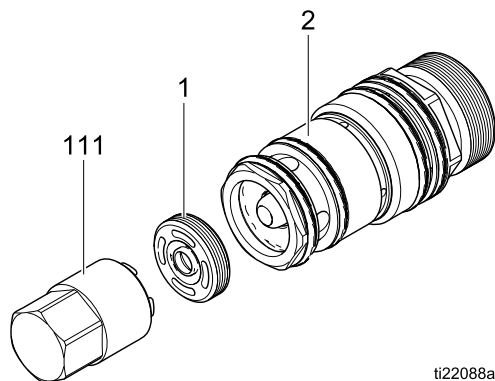
Fig. 1: Remove Valve Seat
