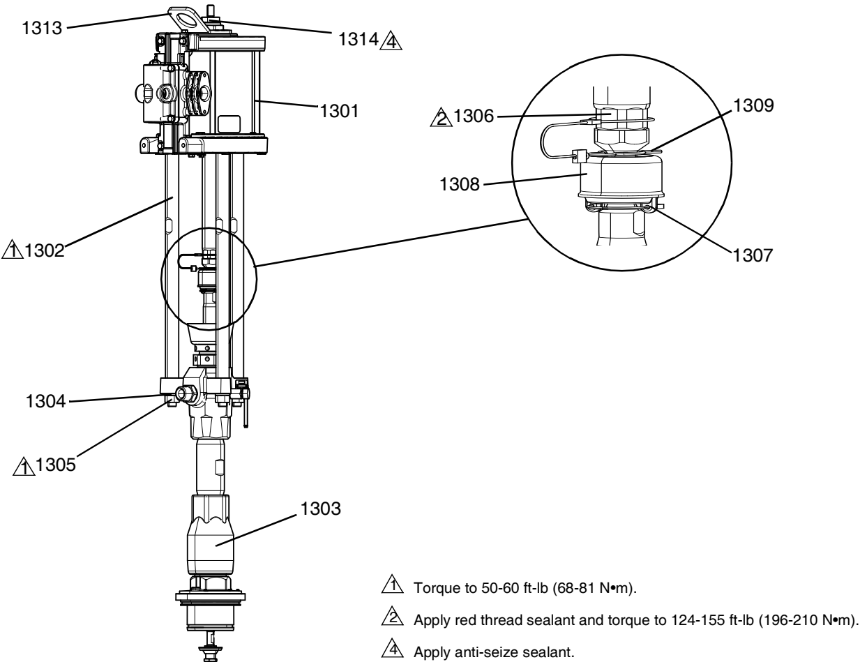
FIG. 20: Pump Assembly Kit
