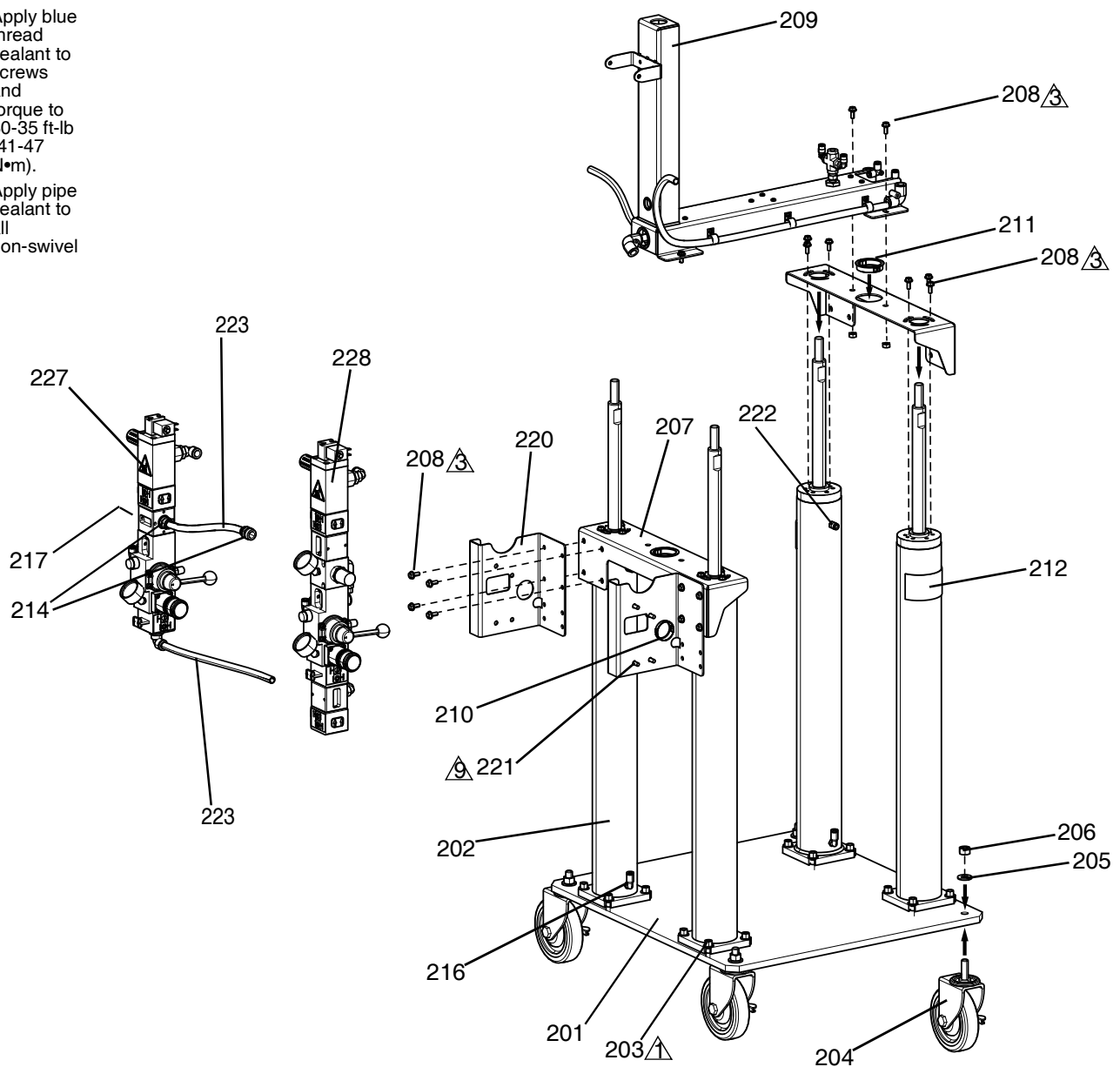
FIG. 3: F4-5 Base - Ram, Dual
