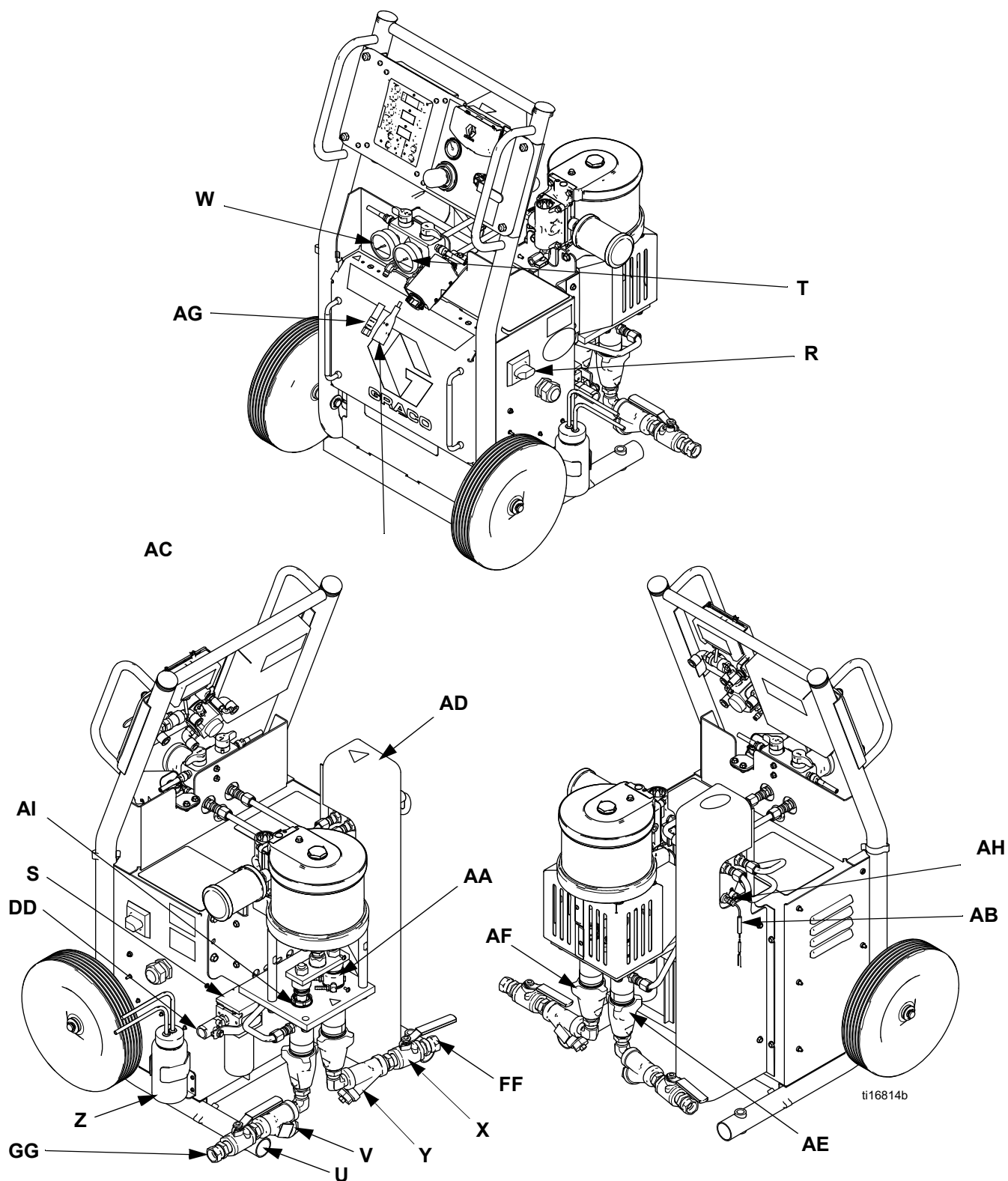
FIG. 3: Installation type
