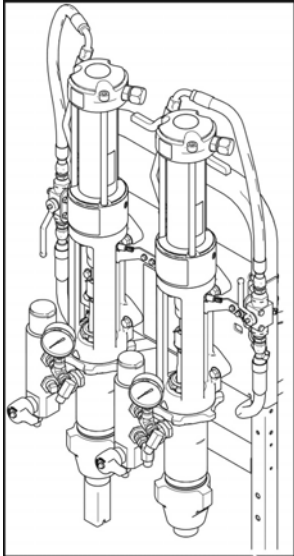
Pump Assembly
