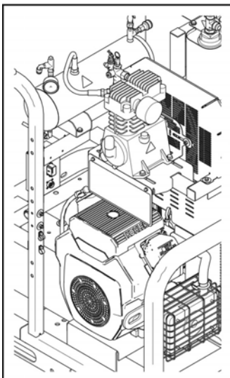
Engine and Compressor Assembly
