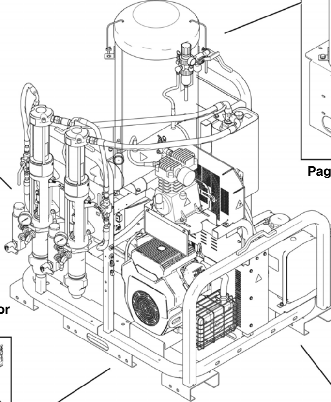
RoadLazer RoadPak Module 24G624, 24G625
