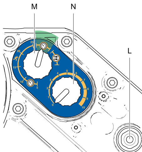
Figure 11 Mode pression
