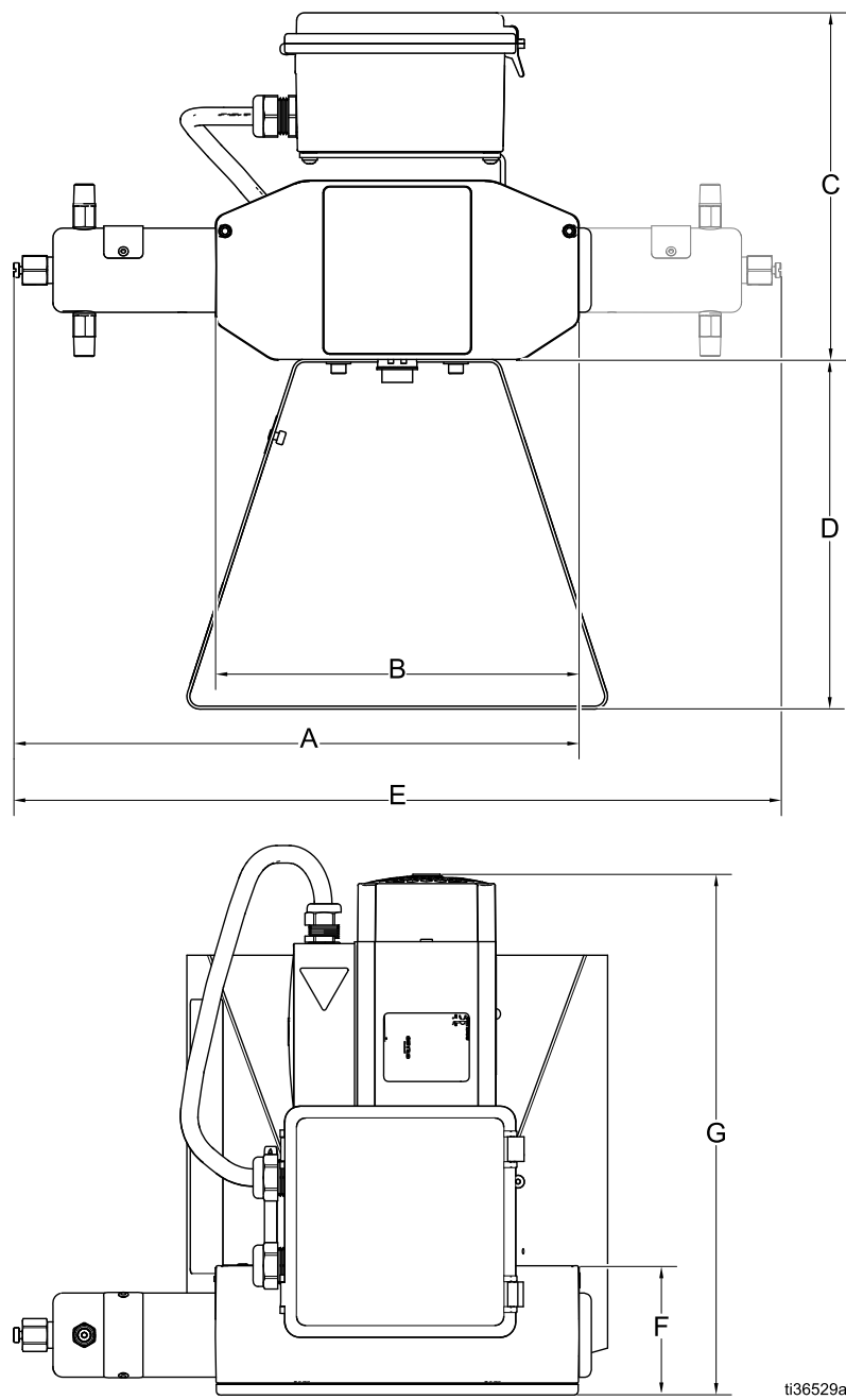
FIG. 14 G-Chem Pump with Harrier AC Dimensions
