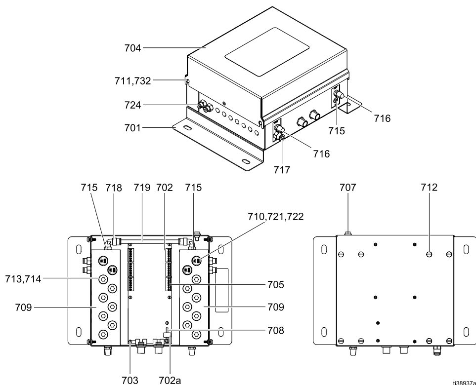
Figure 64 Kontrollmodul – reparation (icke-IS-modell i bild)
