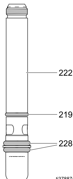
Figure 40 Byta ut isolationsventilens O-ringar
