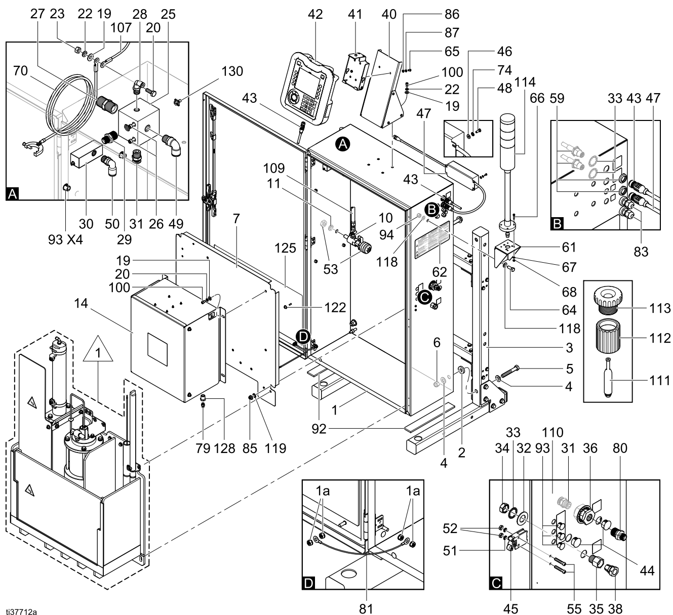
Figure 58 Isolationsskåp
