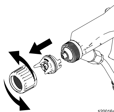
Figure 18 卸下空气帽
