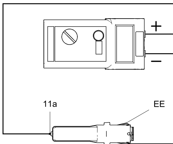
Figure 16 测试供电电源的电阻
