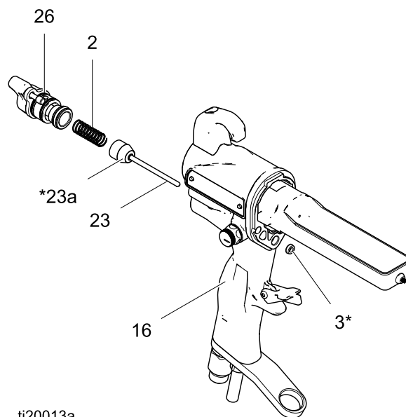
Figure 37 空气阀
