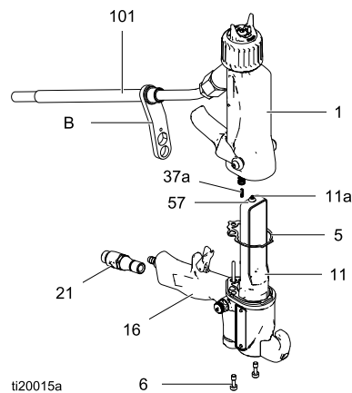
Figure 24 枪筒安装
