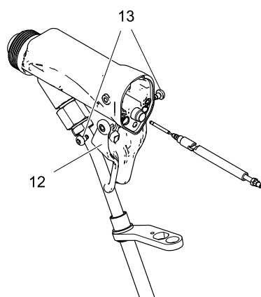
Figure 27 更换流体枪针
