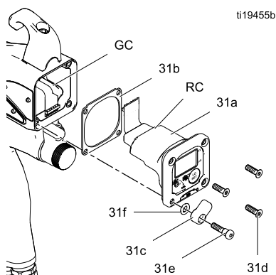
Figure 38 智能模块
