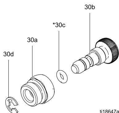
Figure 33 扇形空气调节阀
