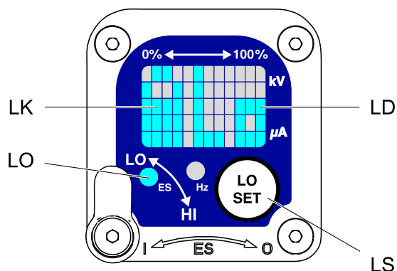
Figure 9 低压锁定屏幕
