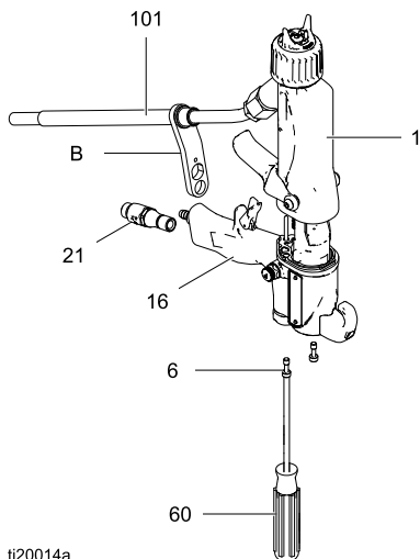
Figure 23 枪筒拆卸
