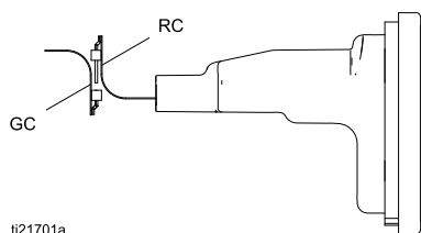
Figure 39 对齐带状电缆
