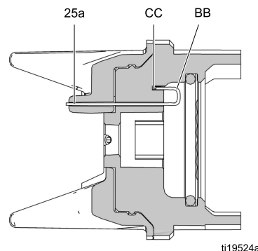
Figure 22 更换电极
