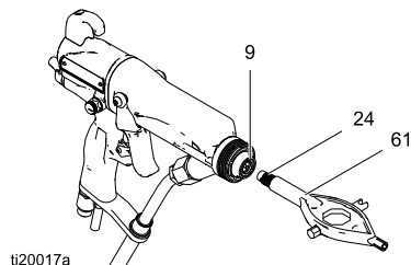
Figure 21 更换流体座外壳
