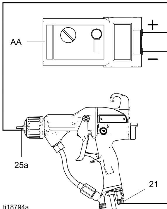
ti18794a Figure 15 测试喷枪的电阻
