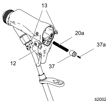
Figure 25 卸下帽子和弹簧
