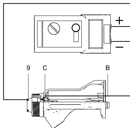
Figure 17 测试枪筒电阻
