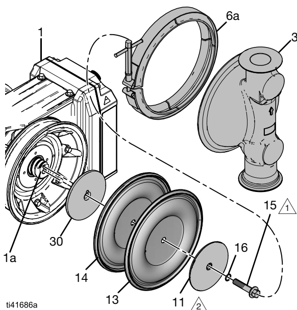
FIG. 17: Remontere standardmembraner (hygienemodell vist)
