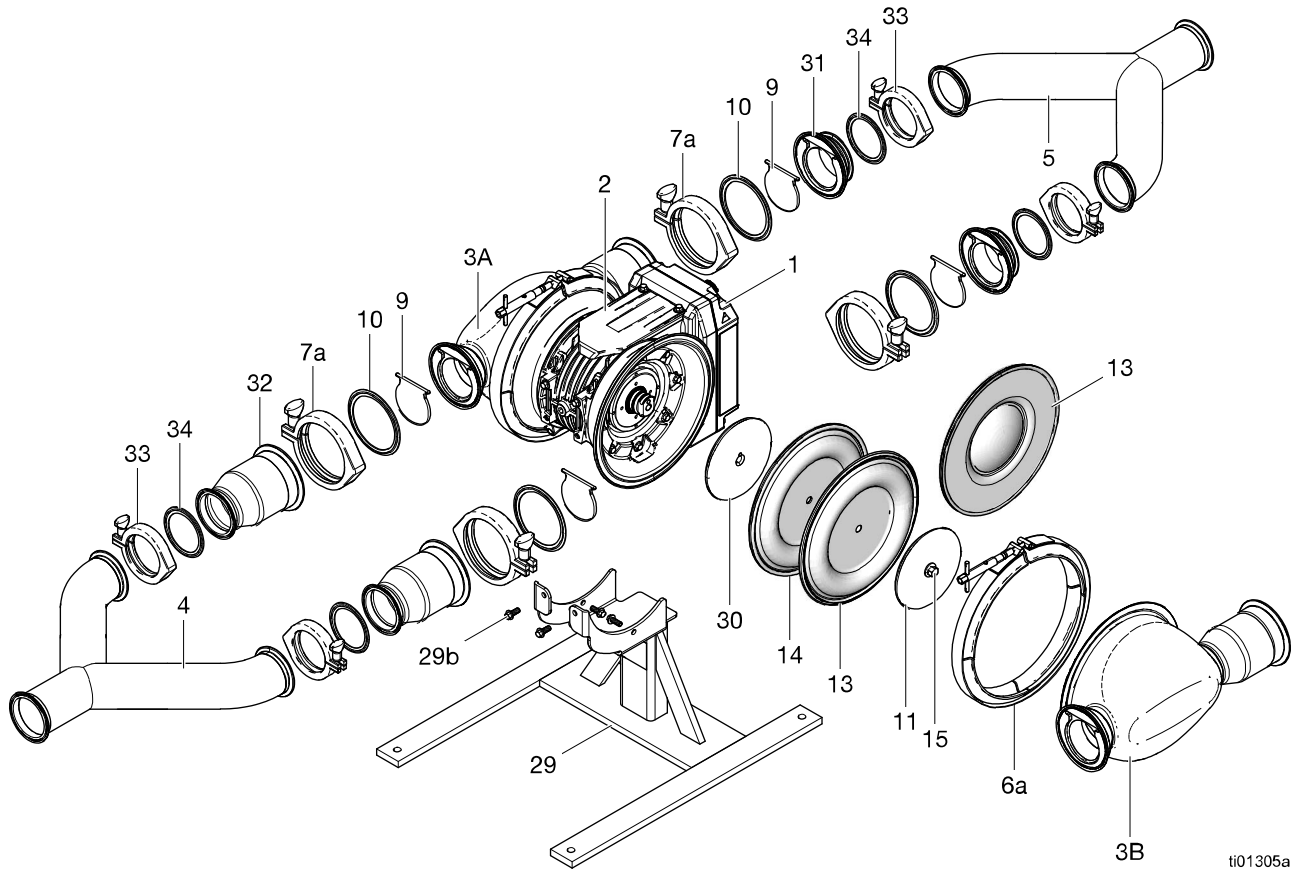
h120 (QHF) High Sanitation (HS) Horizontal Flapper model shown (SSE/SSG)
