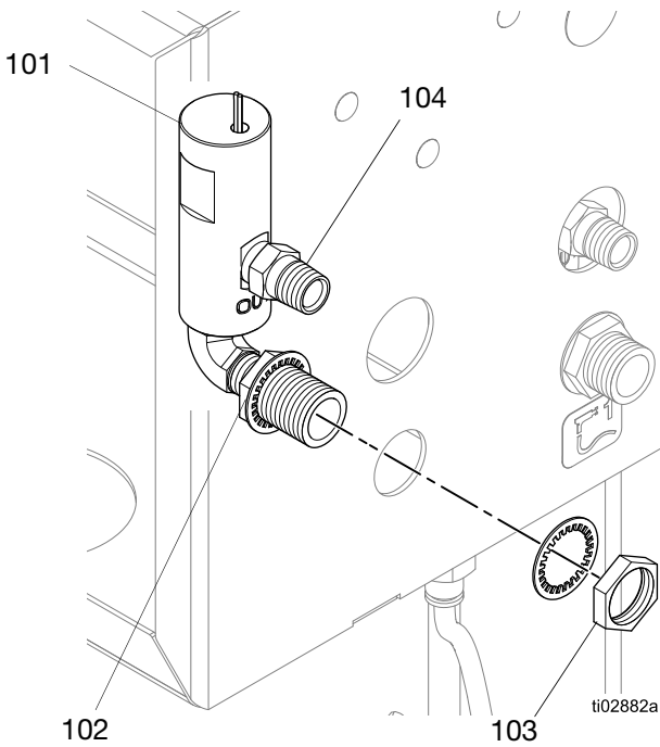
FIG. 2: Install Solvent Flow Switch
