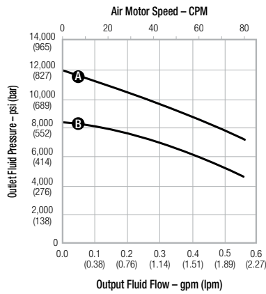
Dyna-Star 120:1 Pump Performance Curve
