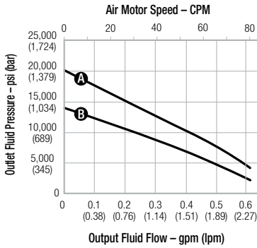
Dyna-Star 120:1 Pump Performance Curve
