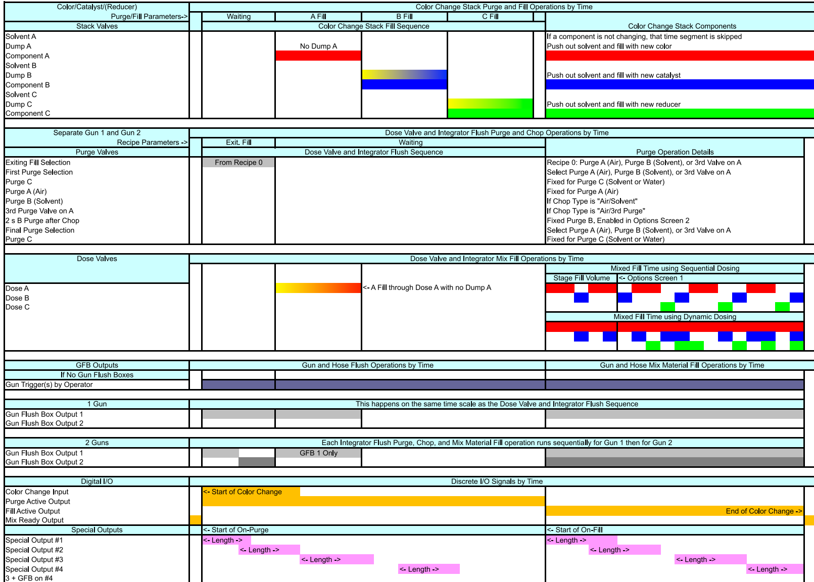
FIG. 76: ProMix 3KS Recipe Fill Chart #5 0 to Y
