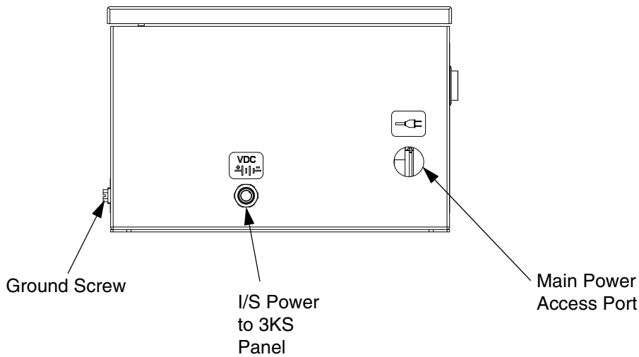
FIG. 6. Connections and AC Power Switches
