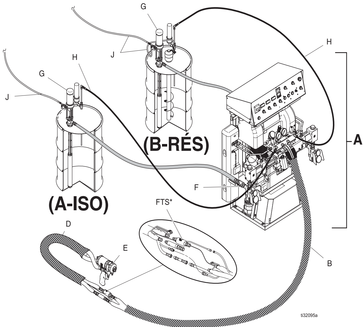
FIG. 2: Installation type
